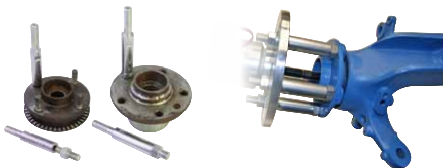
Pushing out the drive shaft, mechanically on the workbench
