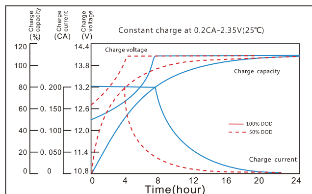
Charging characteristic
