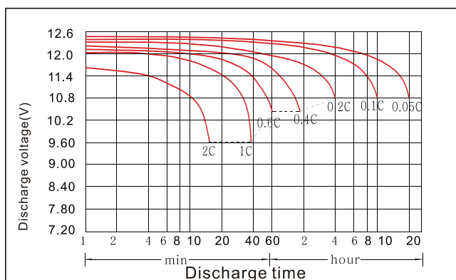
Discharge characteristic
